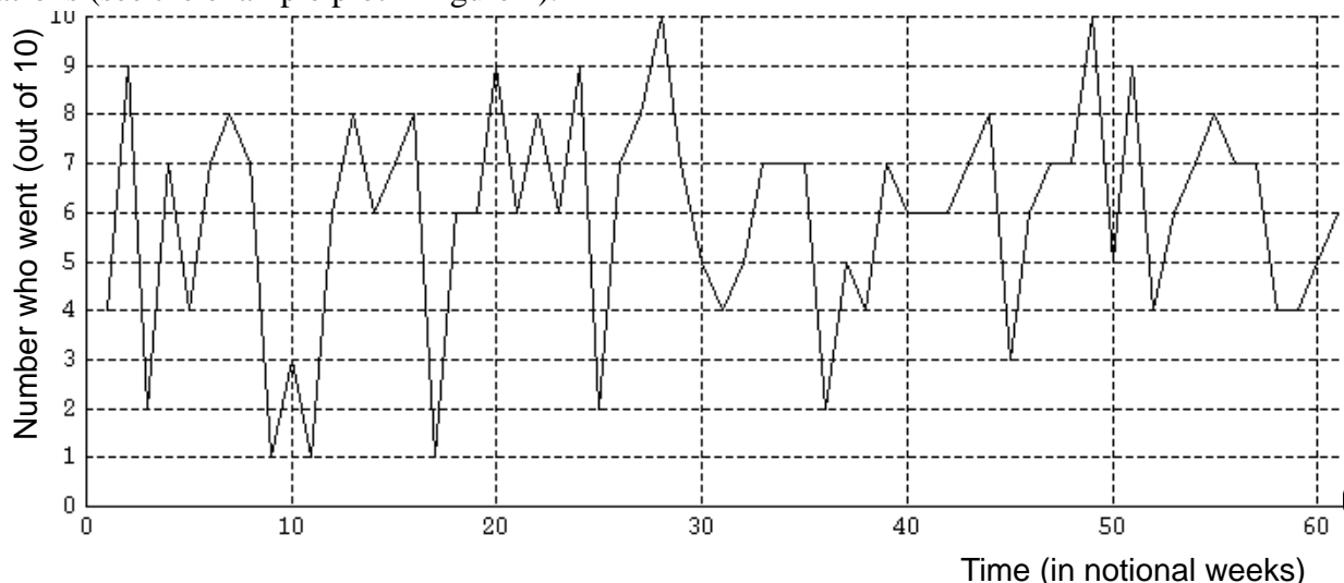
Figure 2: Number of people going to El Farol's each week in a typical run
